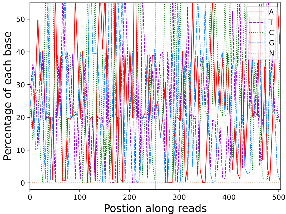
Base percentage along reads (R10524)
